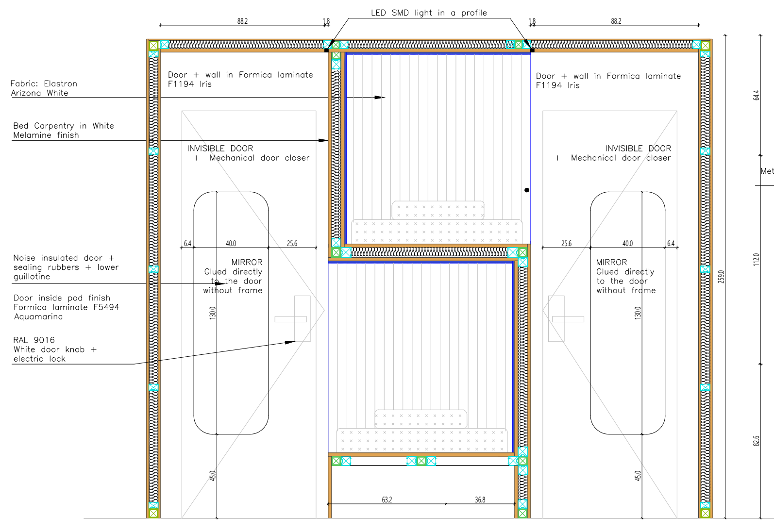
Section 2-2 Scale 1:25
