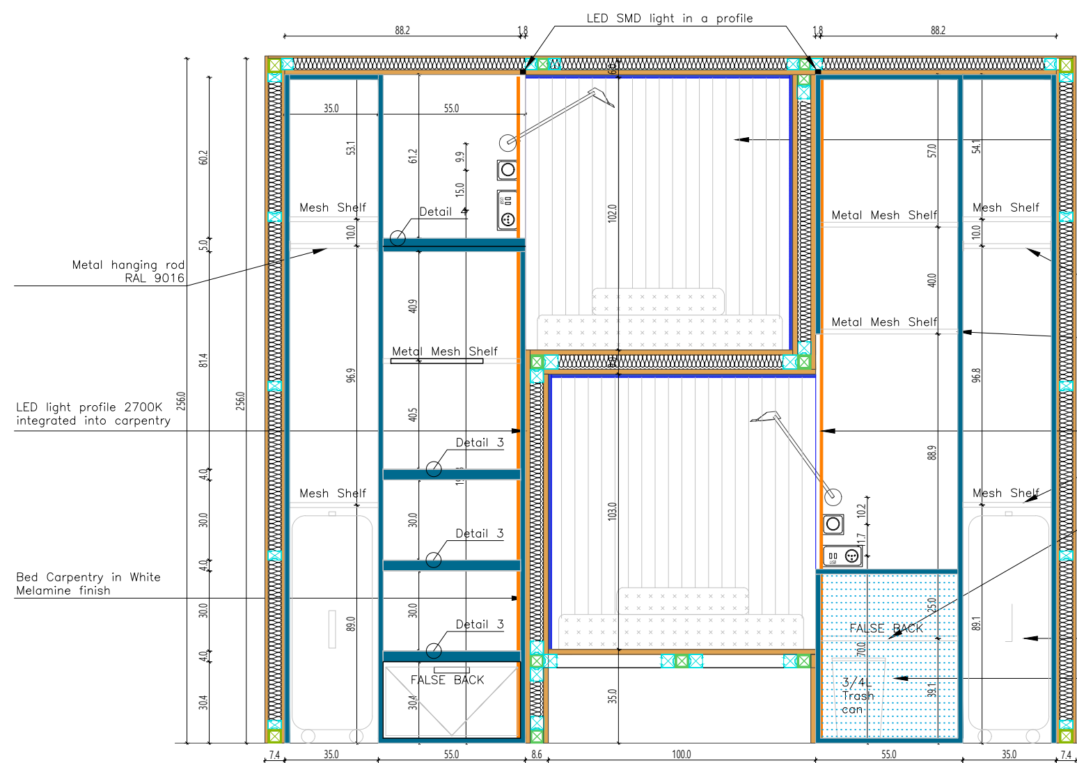
Section 1-1 Scale 1:25
