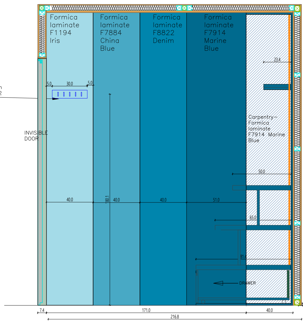
Section 3-3 Scale 1:25
