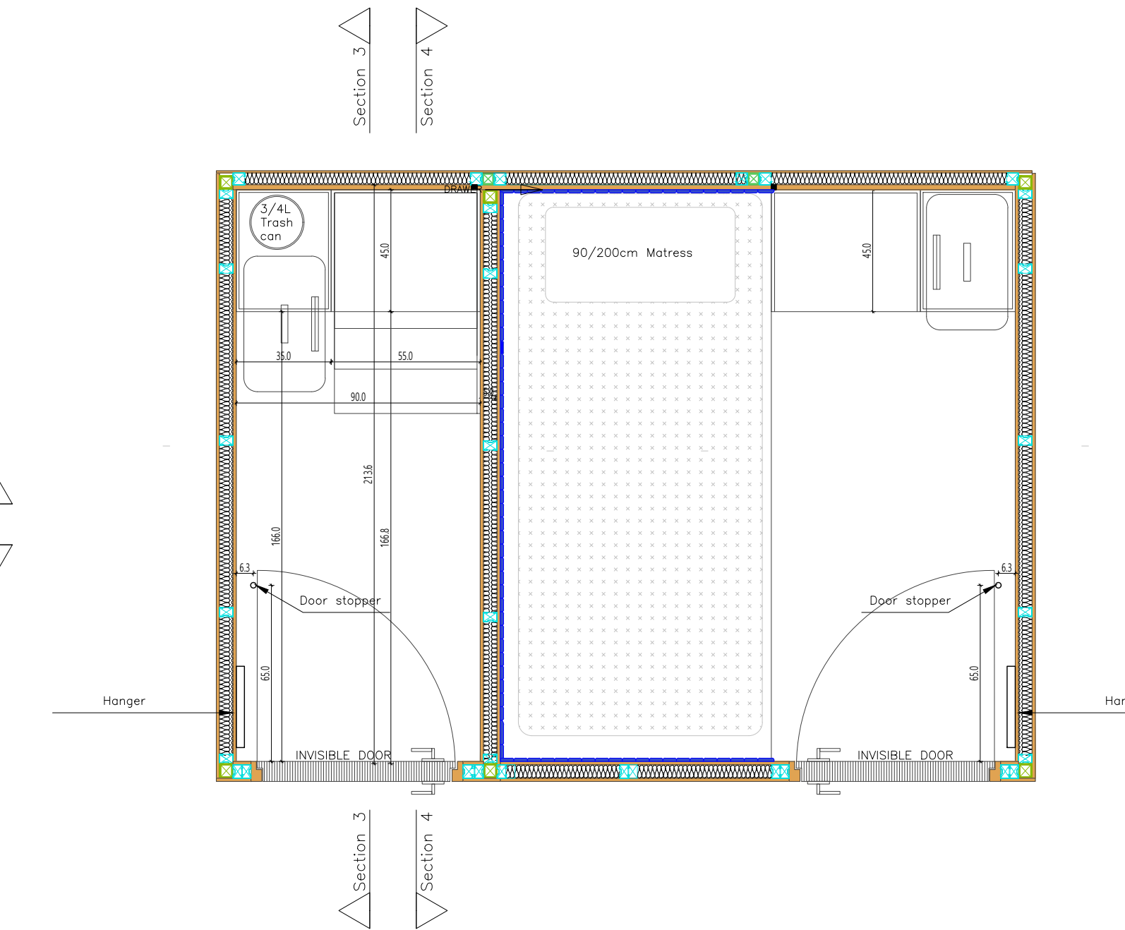
Plan; Level +1.20 Scale 1:25
