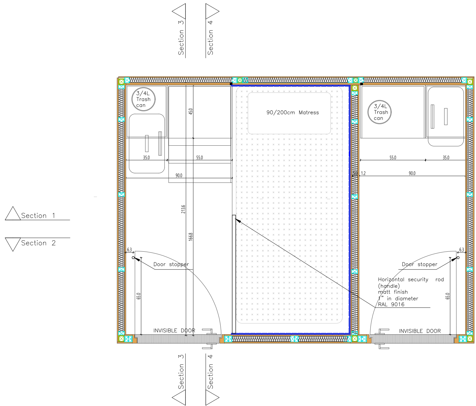
Plan; Level +2.20 Scale 1:25
