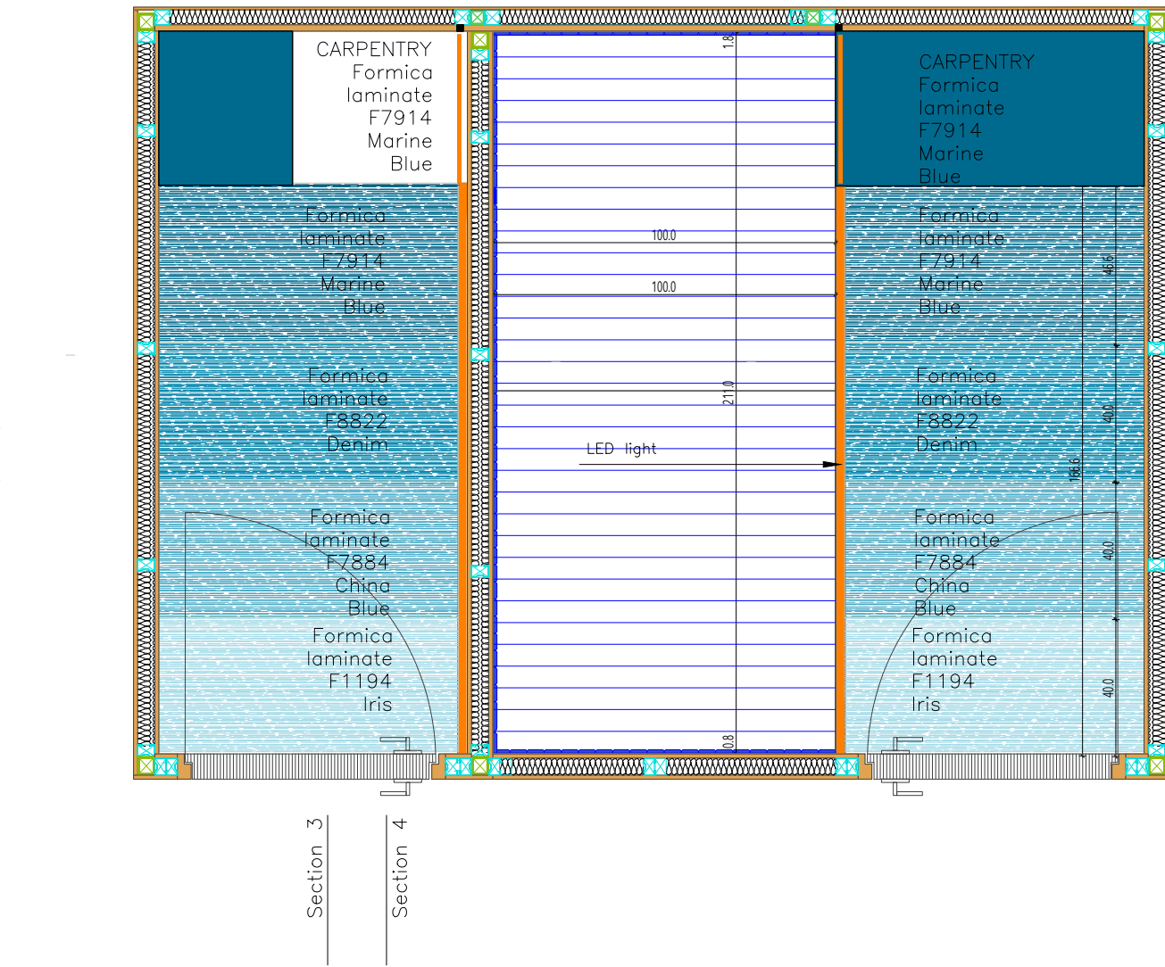
Plan; Ceiling Scale 1:25
